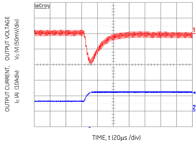
Figure 34. Transient Response to Dynamic Load Change from 50% to 100% at 12Vin, Cout=5x47µF, CTune=1500pF & RTune=330ohms
