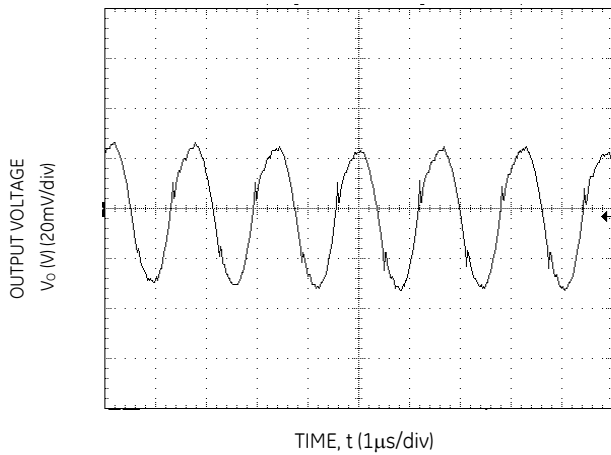
Figure 33. Typical output ripple and noise (Co=22µF ceramic, Vin = 12V, Io = Io,max.).
