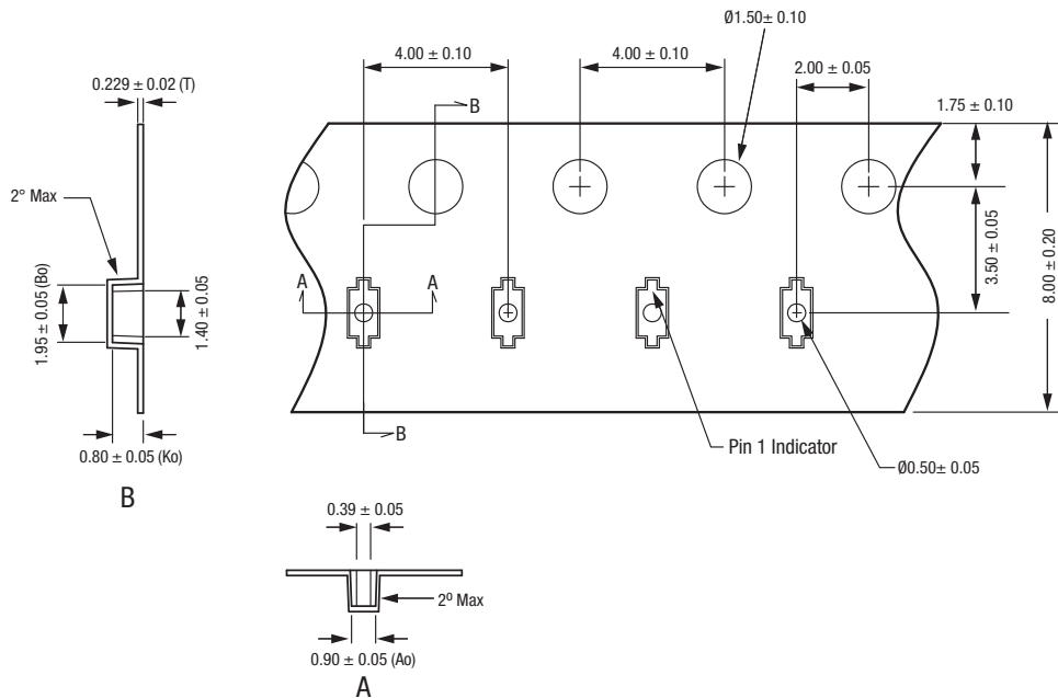
Figure 5. SC-79 Package Dimension Drawing
