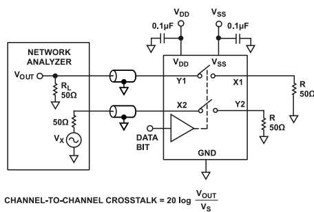
Figure 32. Channel-to-Channel Crosstalk
