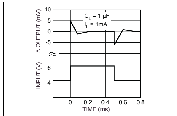
FIGURE 2-17: Line Transient.
