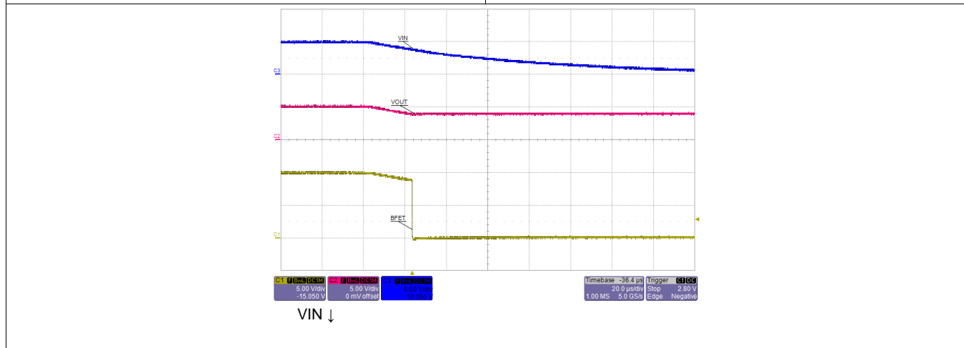
Figure 35. Turnoff Delay to BFET
