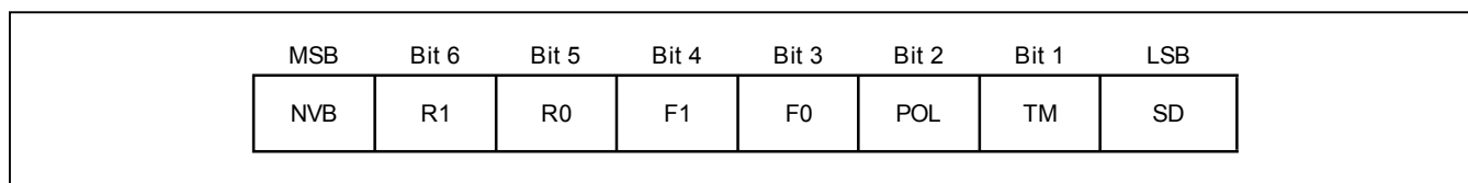
Figure 5. Configuration Register
