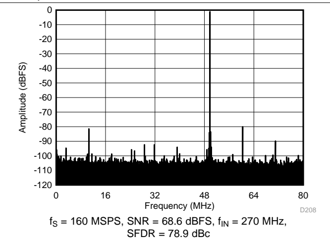
Figure 8. FFT for 270-MHz Input Signal (Dither Off)
