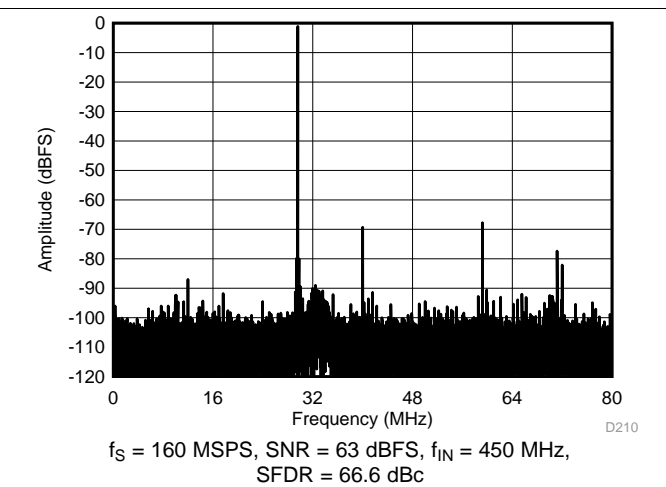
Figure 10. FFT for 450-MHz Input Signal (Dither Off)
