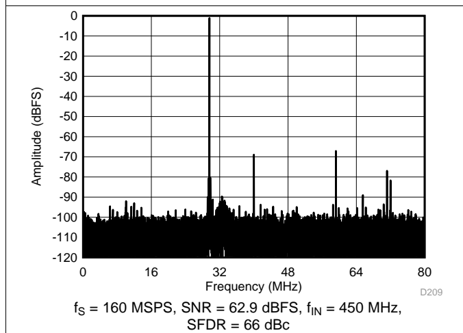
Figure 9. FFT for 450-MHz Input Signal (Dither On)
